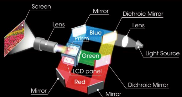
3LCD Projection System
